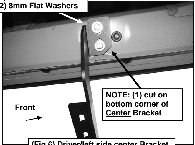
(Fig 6) Driver/left side center Bracket
