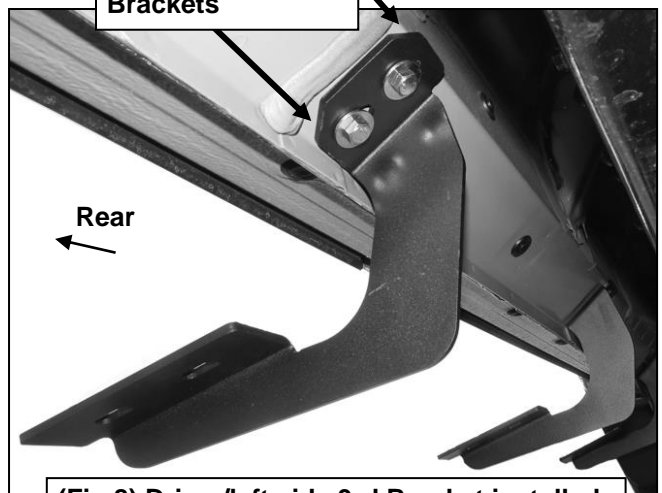
(Fig 8) Driver/left side 3rd Bracket installed
