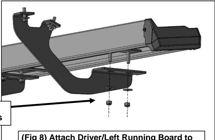
(Fig 8) Attach Driver/Left Running Board to the Mounting Brackets
