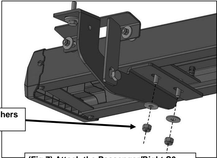
(Fig 7) Attach the Passenger/Right S6 Running Board to the Mounting Brackets
