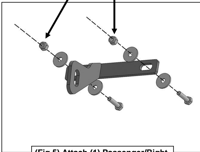
(Fig 5) Attach (1) Passenger/Right Support Bracket to the (2) holes in the pinch trim in the front location
