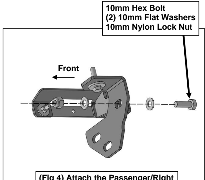
(Fig 4) Attach the Passenger/Right Support Bracket to the pinch weld and the Mounting Bracket
