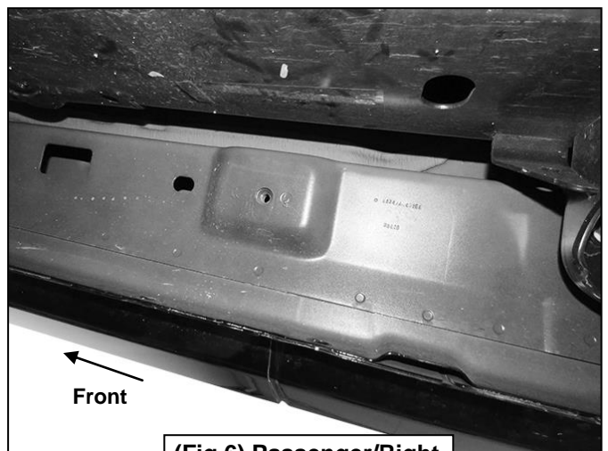
(Fig 6) Passenger/Right 2nd mounting location
