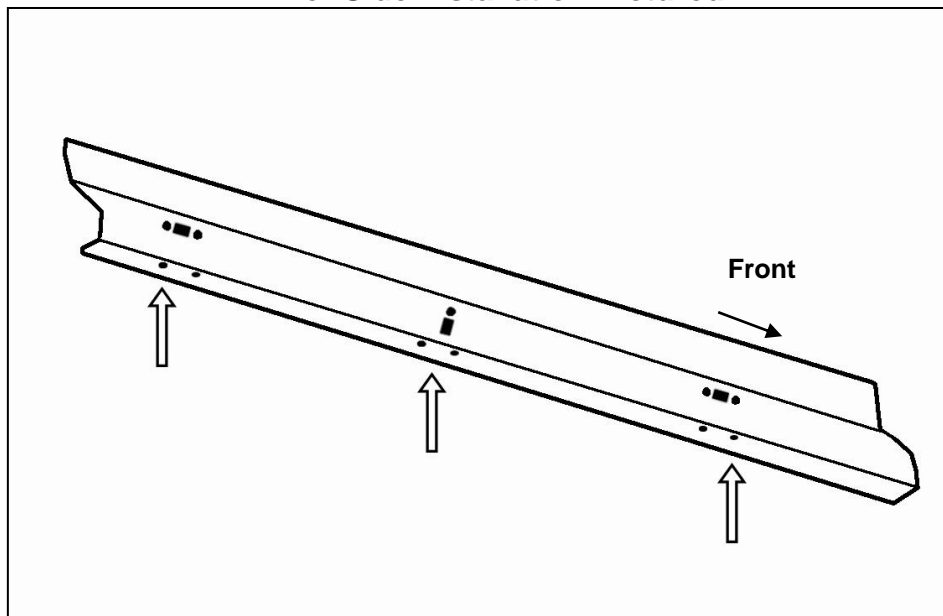
(Fig 1) Driver/left mounting locations illustrated from back of rocker panel
