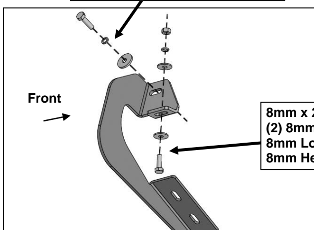
(Fig 7) Driver/left Center Bracket installed
