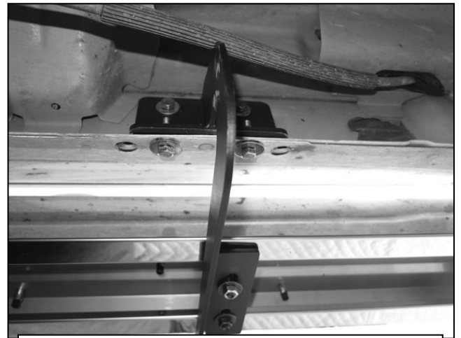
(Fig 11) Driver/left front complete installation
