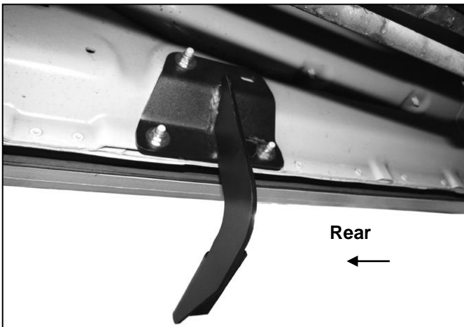
(Fig 7) Driver/left Side rear Bracket installed
