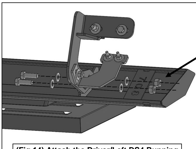
(Fig 14) Attach the Driver/Left DS4 Running Board to the (3) Mounting Brackets
