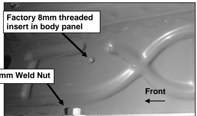
(Fig 2) Passenger/Right Front mounting location
