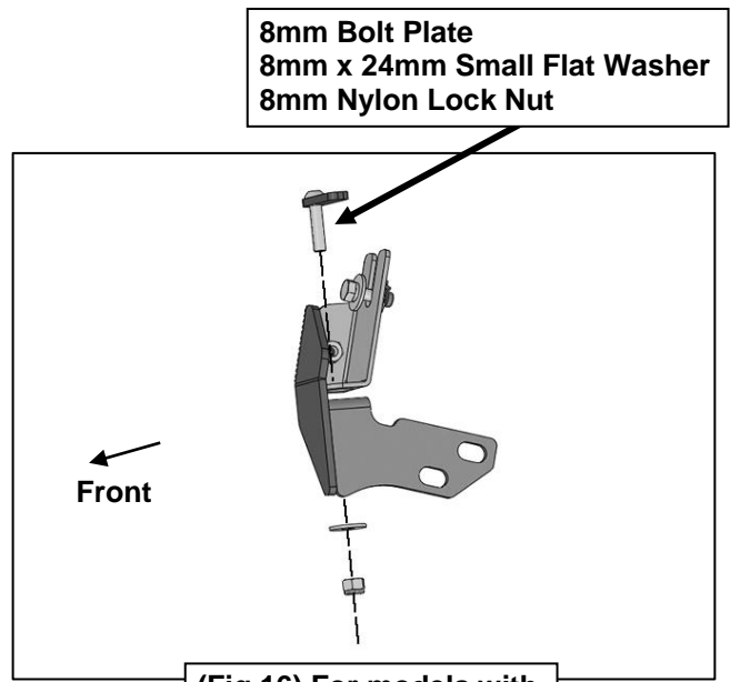
(Fig 16) For models with a hole in the pinch weld
