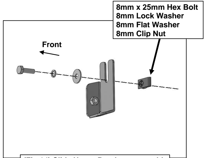
(Fig 14) Slide Upper Bracket over weld nut if equipped-also see Figure 2
