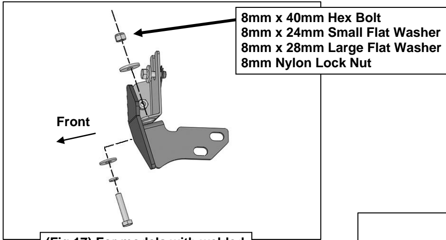
(Fig 17) For models with welded nut in the pinch weld
