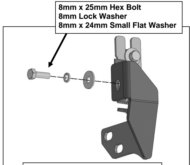
(Fig 18) Secure the side of the Lower Bracket to the Upper Bracket
