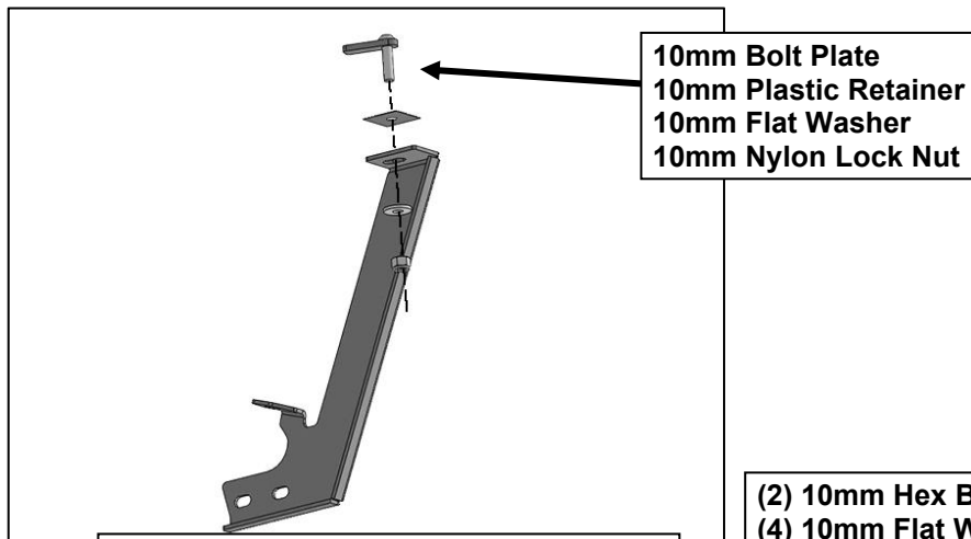
(Fig 9) Attach (1) Driver/Left Rear Mounting Bracket per 10mm Bolt Plates
