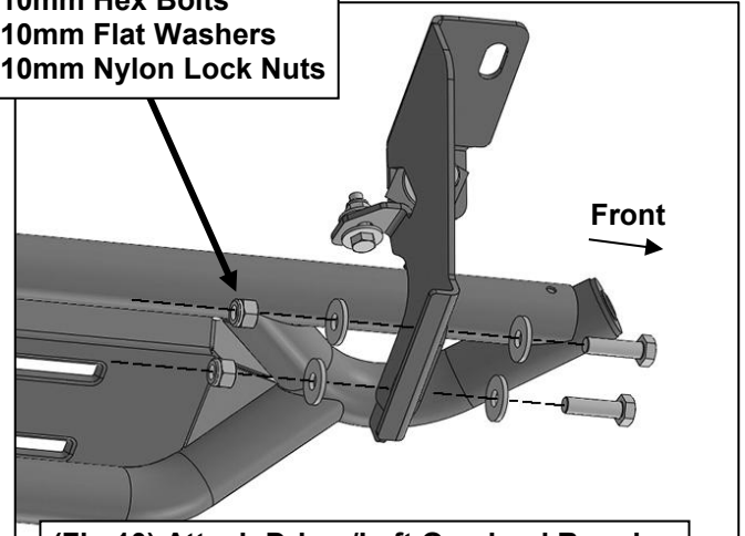
(Fig 10) Attach Driver/Left Overland Running Board to the (4) Mounting Brackets
