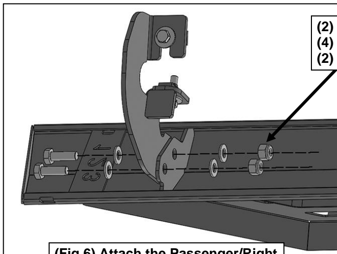
(Fig 6) Attach the Passenger/Right Running Board to the rear faces of the Mounting Brackets
