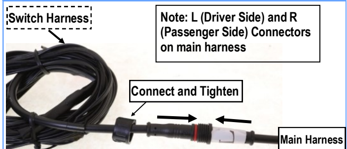
(Fig 8) Connect the Switch Harness to the Main Harness
