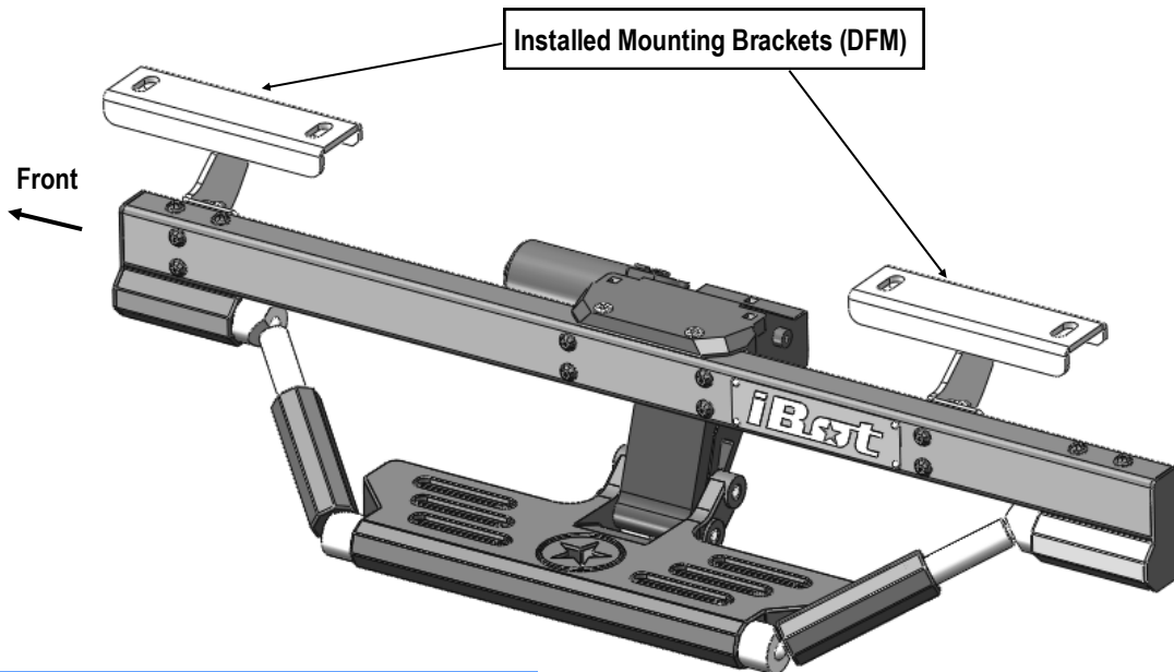
(Fig 2) Driver Side Mounting Brackets and Step Bar Assembly
