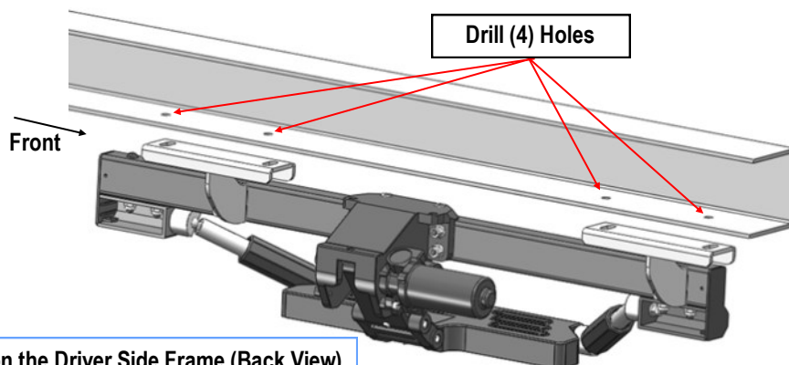
(Fig 3) Mark and Drill Mounting Holes on the Driver Side Frame (Back View)
