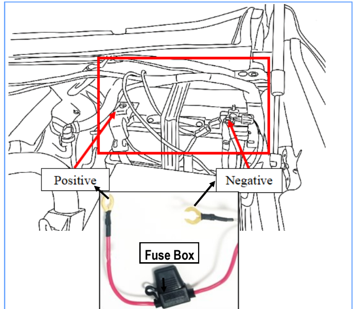
(Fig 6) Connect the Main Harness to the Battery Terminals
