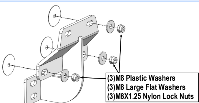
(Fig 3) Driver Front Mounting Bracket Installation
