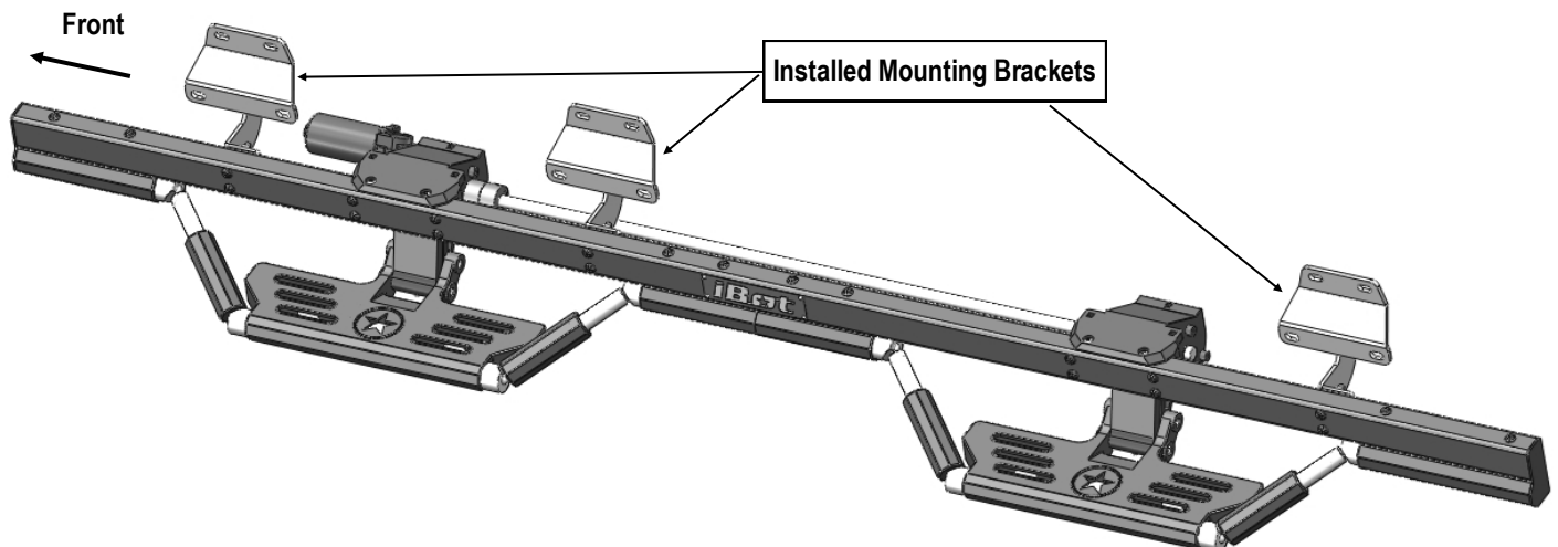
(Fig 14) Driver Side Step Bar Installation
