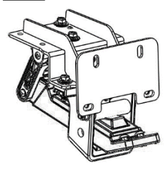
Passenger Rear Bracket Assembly
