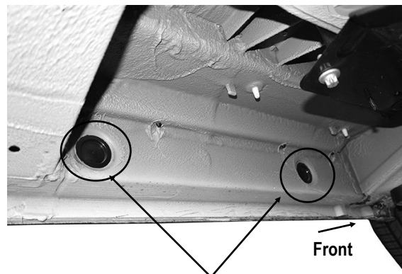
(Fig 12) Driver Side Front & Rear Mounting Locations
