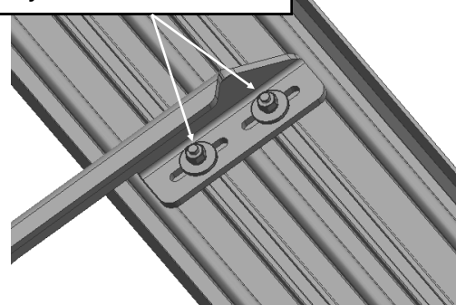
(Fig 9) Running Board Installed Onto Mounting Bracket (Example)
