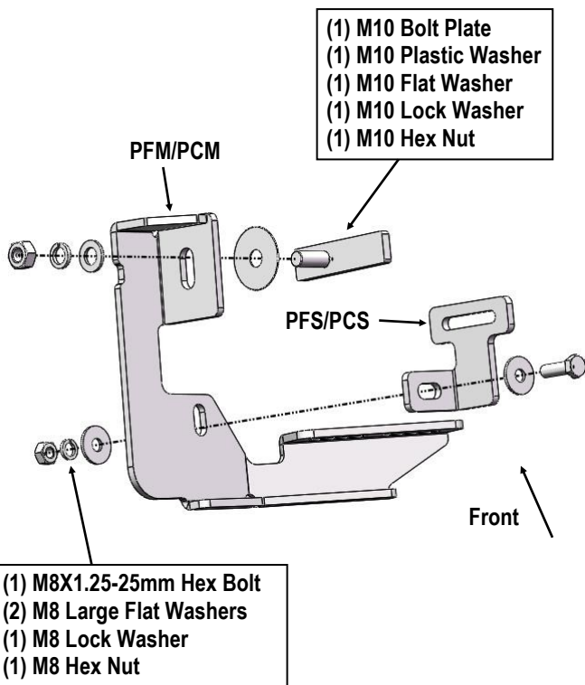
(Fig 3) Passenger Front Mounting Bracket (PFM/PCM) and Passenger Front Support Bracket (PFS/PCS) Installation
