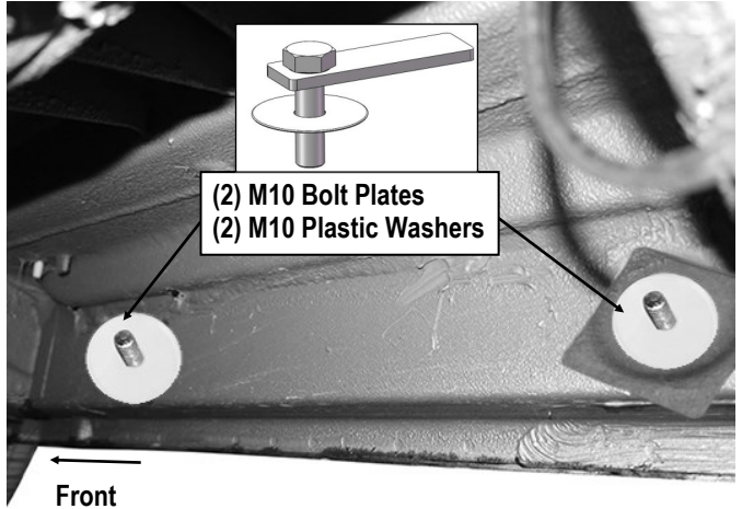
(Fig 2) M10 Bolt Plate Installed (On Passenger Side Front & Center Mounting Location)
