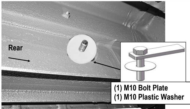
(Fig 5) Passenger Side Rear Mounting Location
