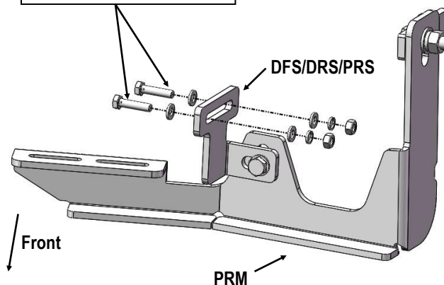
(Fig 11) Attach Support Bracket To Pinch Weld
