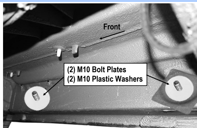
(Fig 5) M10 Bolt Plate Installed (On Passenger Side Front & Center Mounting Location)
