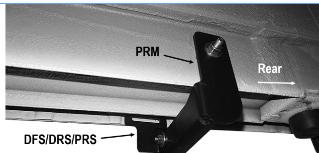
(Fig 10) Passenger Rear Bracket Installed
