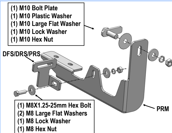
(Fig 9) Passenger Rear Mounting Bracket (PRM) and Passenger Rear Support Bracket (DFS/DRS/PRS) Installation
