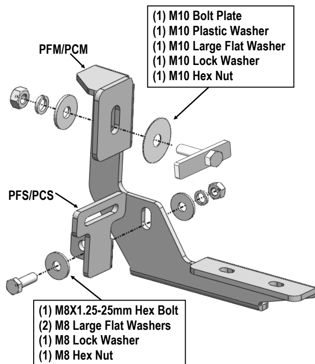
(Fig 6) Passenger Front Mounting Bracket (PFM/PCM) and Passenger Front Support Bracket (PFS/PCS) Installation
