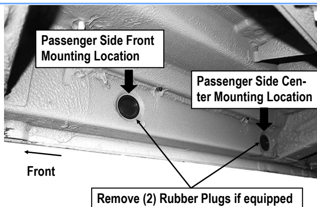
(Fig 4) Passenger Side Front & Center Mounting Locations
