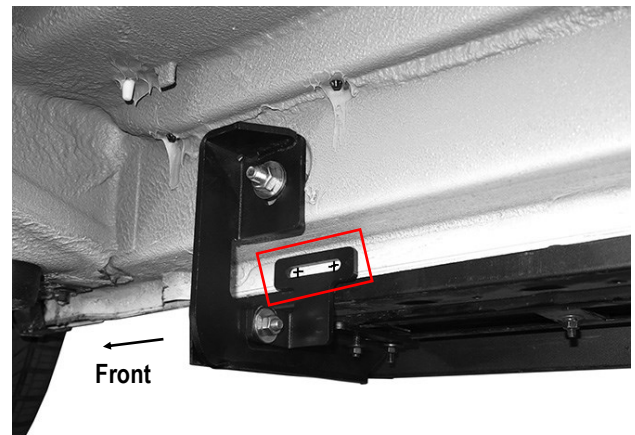
(Fig 13) Mark location of each Support Bracket onto pinch weld before drilling
