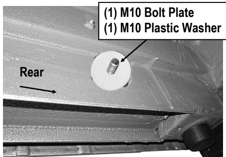
(Fig 8) Passenger Side Rear Mounting Location
