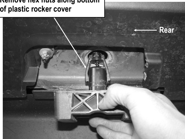
(Fig 2) Remove Plastic Plug
