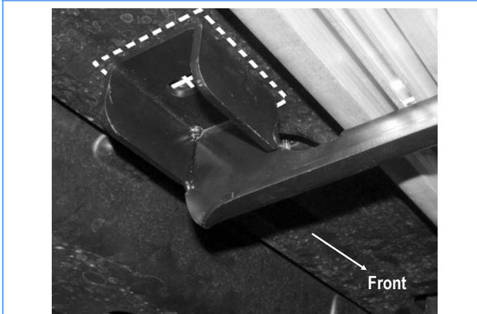
(Fig 9B) Hold the Bracket in place with the slot in the Bracket (Picture For Reference Only)
