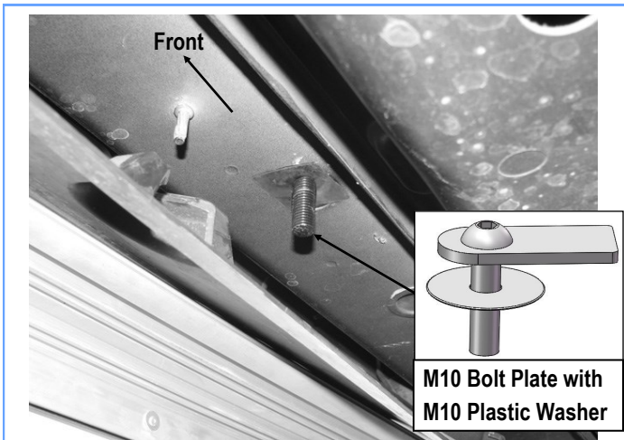
(Fig 8) Passenger Side Center Mounting Location
