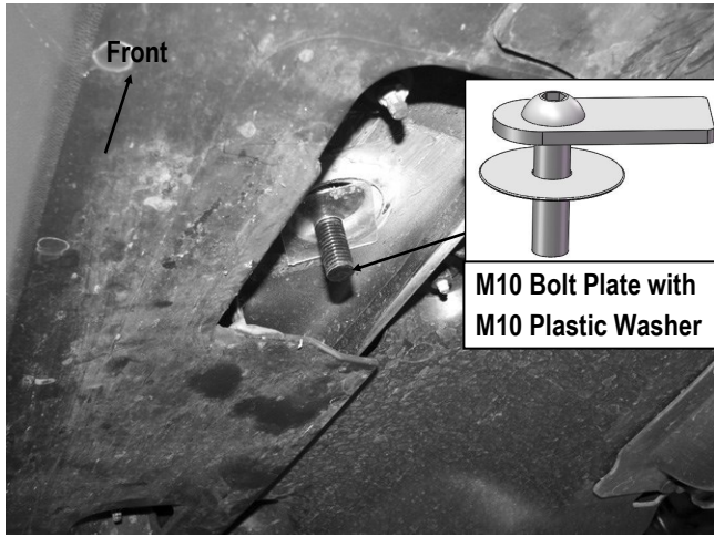
(Fig 4) Passenger Side Front Mounting Location
