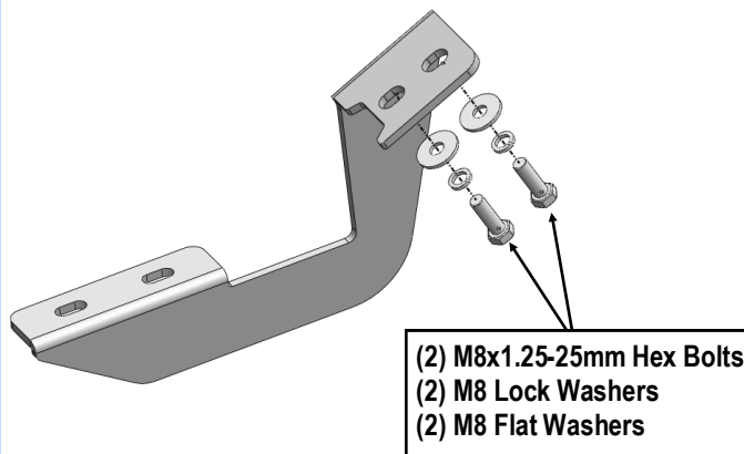
(Fig 4) Driver Center Mounting Bracket Installation
