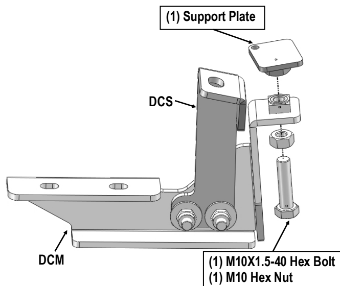
(Fig 11) Driver Side Center Mounting Bracket Installation
