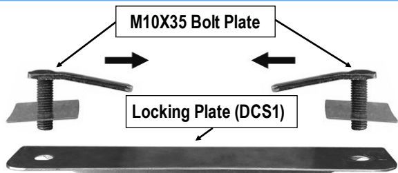
(Fig 8C) Install Bolt Plates With Plates Pointing Towards Each Other
