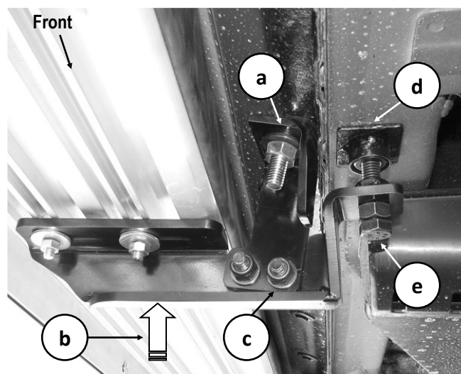
(Fig 18) Driver Side Center Mounting Bracket Installed
