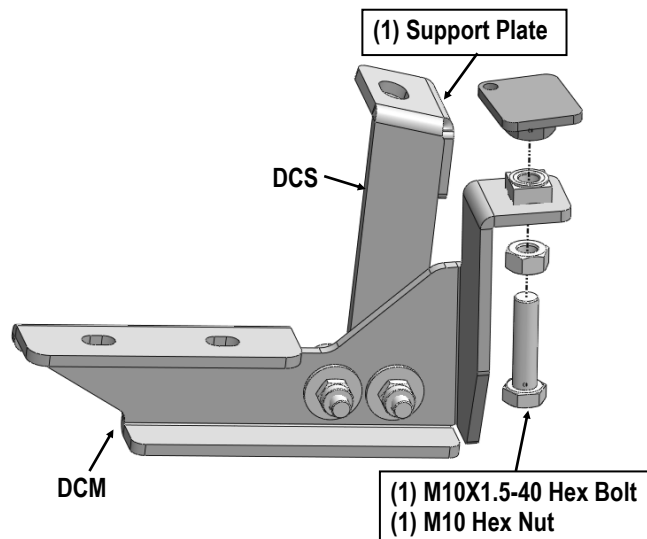
(Fig 11) Driver Side Center Mounting Bracket Installation
