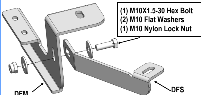
(Fig 5) Driver Side Front Bracket Assembly
