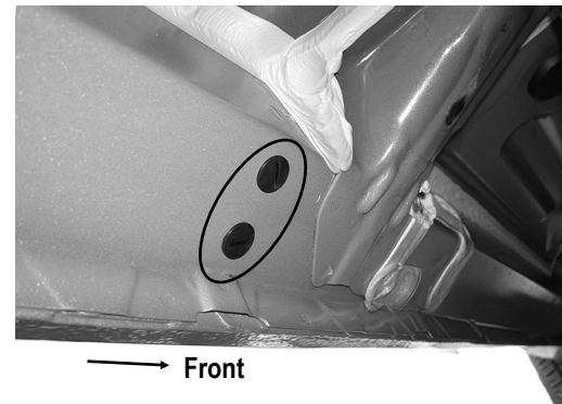
(Fig 3) Example of Driver Side Center & Rear Mounting Location
