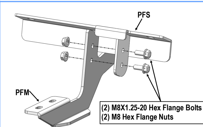
(Fig 2) Passenger Front Mounting Brackets Assembly
