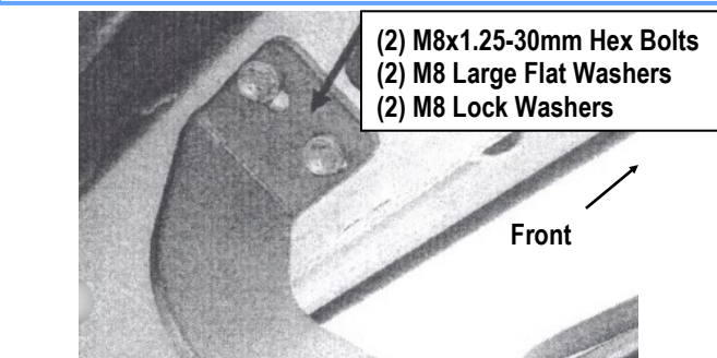
(Fig 2) Driver Side Center Mounting Bracket Installed
