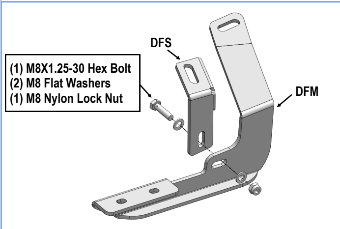
(Fig 6) Driver Side Front Bracket Assembly
