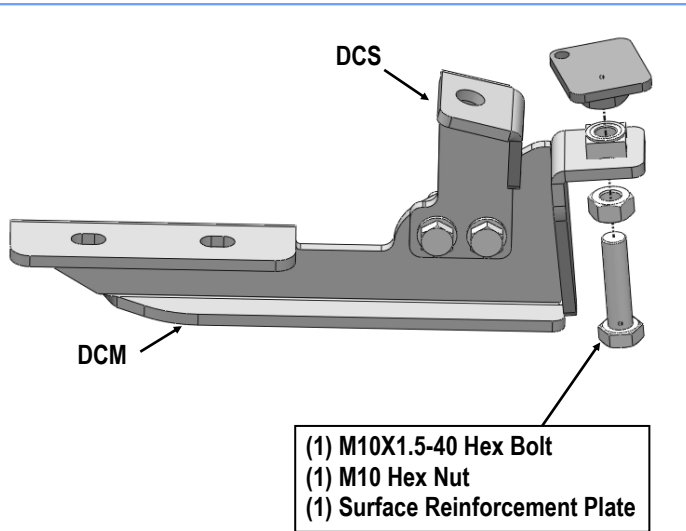
(Fig 12) Driver Side Center Mounting Bracket Installation
