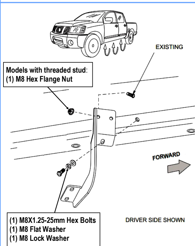
(Fig 3) Models With Threaded Stud Bracket Installed
