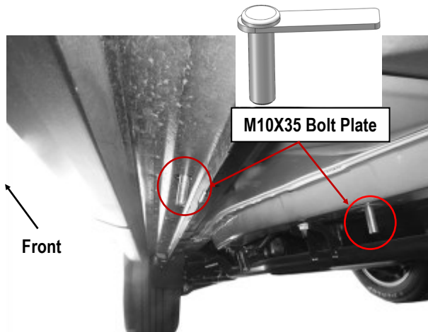
(Fig 6) Insert (2) M10X35 Bolt Plates (Passenger Side Center Mounting Location)
