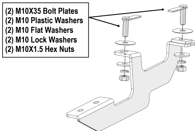
(Fig 3) Passenger Front Mounting Bracket Installation
