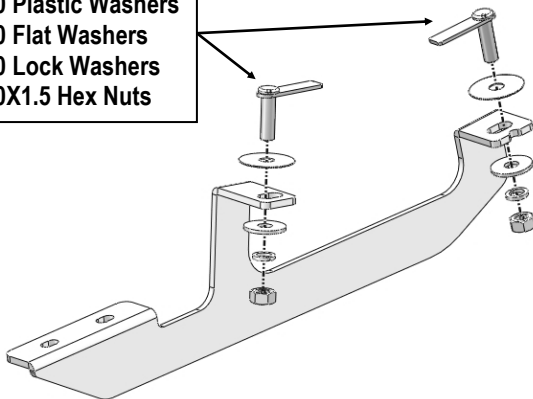
(Fig 7) Passenger Center Mounting Bracket Installation
