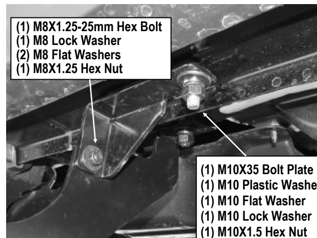
(Fig 12) Passenger Rear Support Bracket Installation
