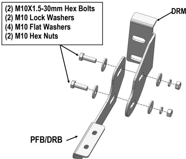
(Fig 6) Driver Rear Mounting Bracket (DRM) and Driver Rear Bar Bracket (PFB/DRB) Assembly
