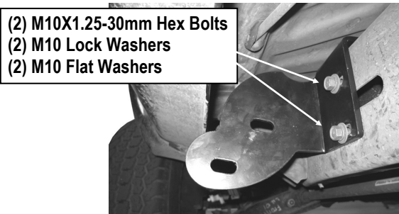
(Fig 2) Driver Front Mounting Bracket (DFM) Installed
