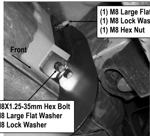
(Fig 3) Driver Side Front Mounting Bracket Installation
