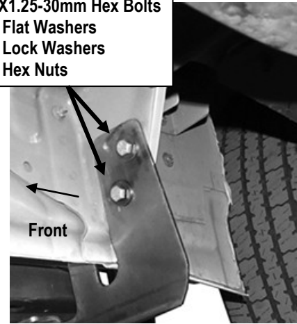
(Fig 14) Passenger Rear Mounting Bracket Complete Installation
