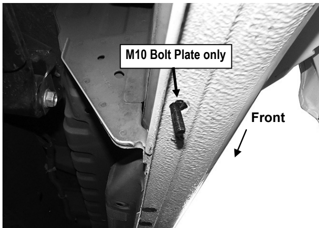
(Fig 8) Passenger Rear Mounting Bracket Location
