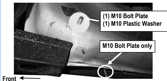
(Fig 3) Passenger Front Mounting Bracket Location
