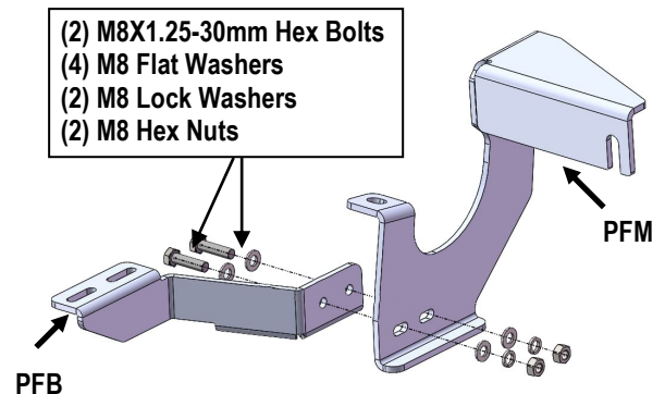
(Fig 2) Passenger Front Mounting Bracket Assembly
