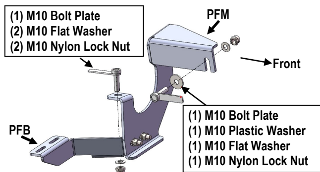
(Fig 4) Assembled Passenger Front Mounting Bracket Installed
