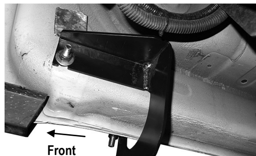
(Fig 5) Passenger Front Mounting Bracket Installed
