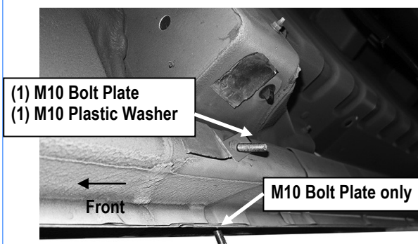
(Fig 6) Passenger Side Center Mounting Location
