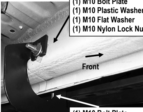
(Fig 16) Driver Front Mounting Bracket (DFM) Installation
