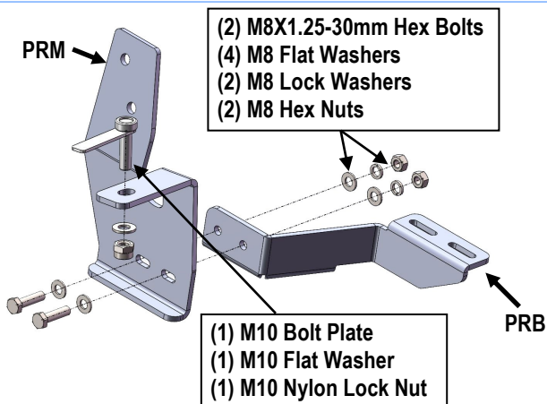
(Fig 9) Passenger Rear Mounting Bracket (PRM) Installation
