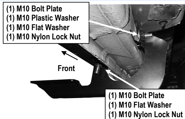
(Fig 7) Passenger Center Mounting Bracket (PCM) Installed
