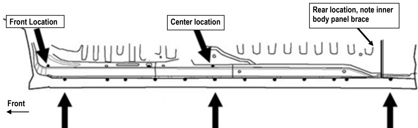
(Fig 1) Passenger Side Mounting Locations
