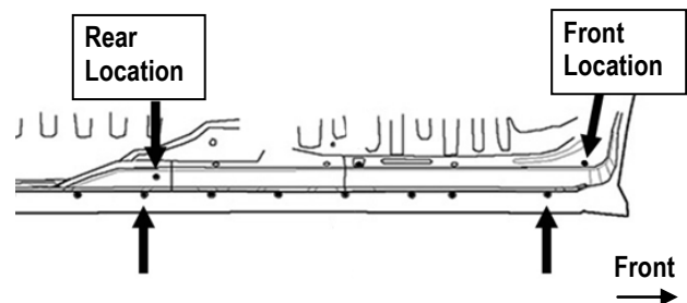
(Fig 15) Driver Side (2) Mounting Locations
