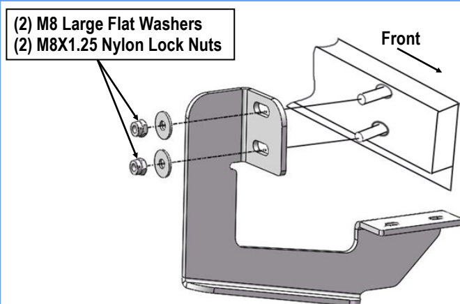
(Fig 2) Driver Side Front Mounting Bracket Installation
