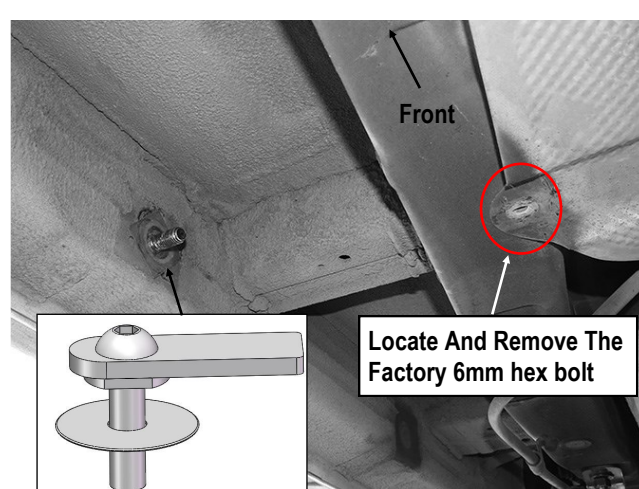
(Fig 4A) M10X40 Short Bolt Plate With M10 Plastic Washer
