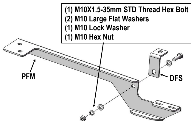
(Fig 4) Passenger Front Support Bracket Assembly
