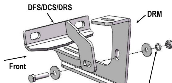
(Fig 7) Driver Center Mounting Bracket Assembly
