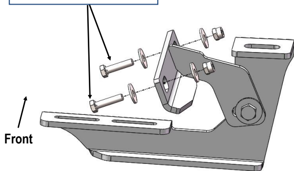
(Fig 9) Driver Front Support Bracket Installed
