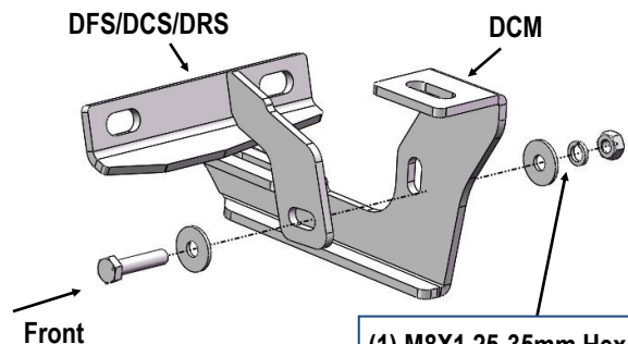
(Fig 6) Driver Front Mounting Bracket Assembly
