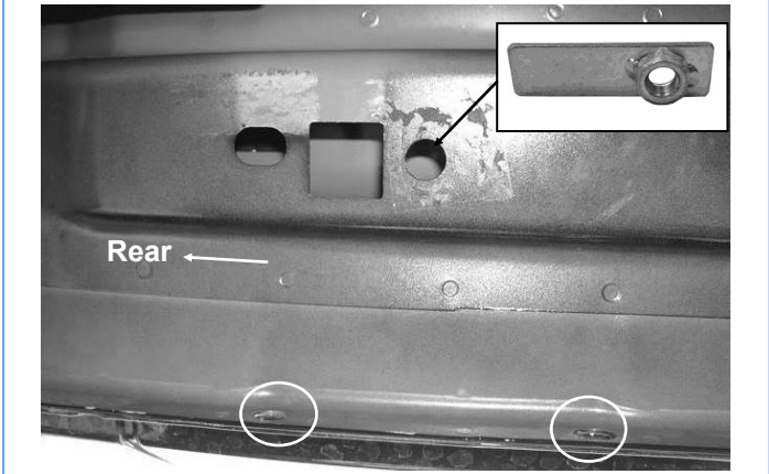
(Fig 3) Driver Side Center & Rear Mounting Location (Vehicles with open mounting location)
