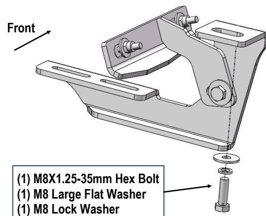
(Fig12) Driver Front Mounting Bracket Installed (Vehicles with factory threaded hole in floor panel)
