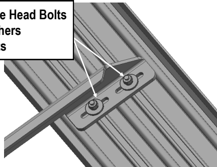
(Fig 14) Running Board Installed Onto Mounting Bracket
