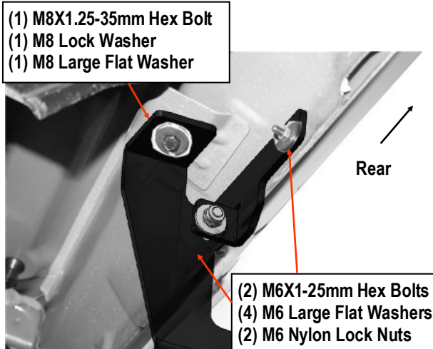
(Fig 11) Passenger Side Rear Brackets Installed
