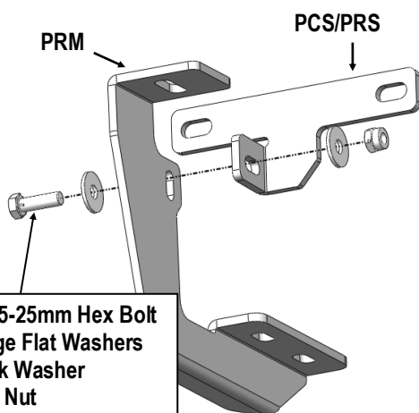
(Fig 10) Passenger Side Rear Brackets Assembly
