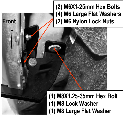
(Fig 5) Passenger Side Front Brackets Installed
