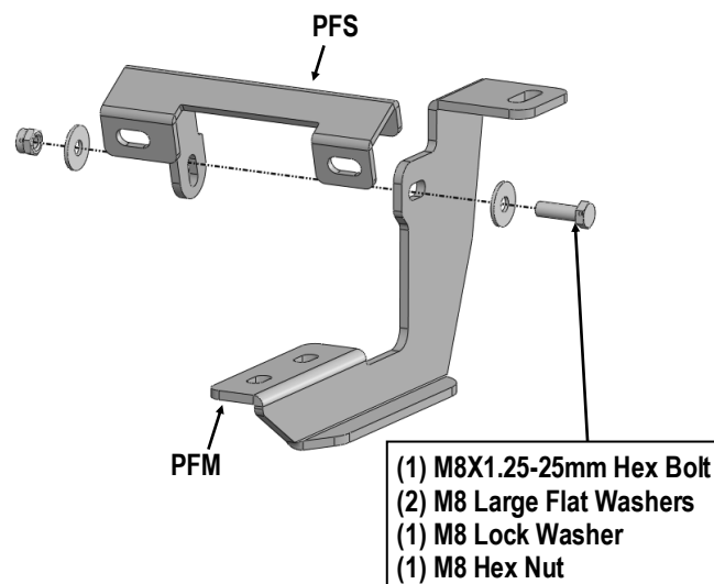
(Fig 3) Passenger Front Brackets Assembly
