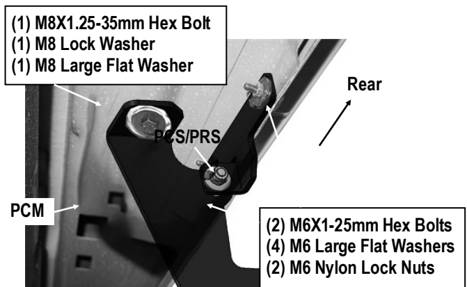
(Fig 9) Passenger Side Center Brackets Installed
