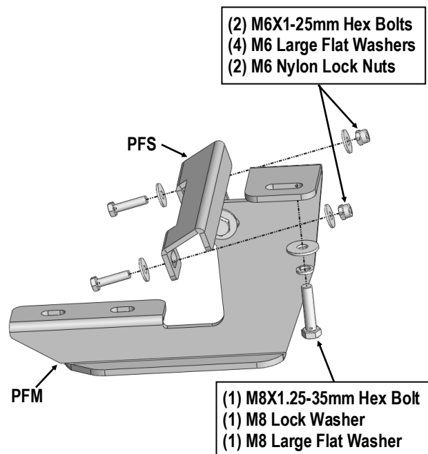
(Fig 4) Passenger Side Front Brackets Installation
