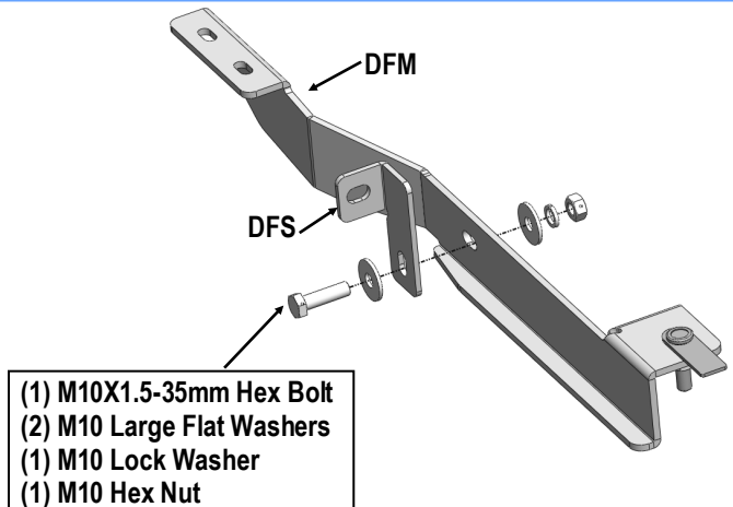
(Fig 3) Driver Front Support Bracket Assembly
