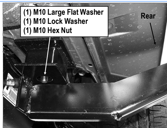
(Fig 5) Driver Rear Mounting Bracket Installation
