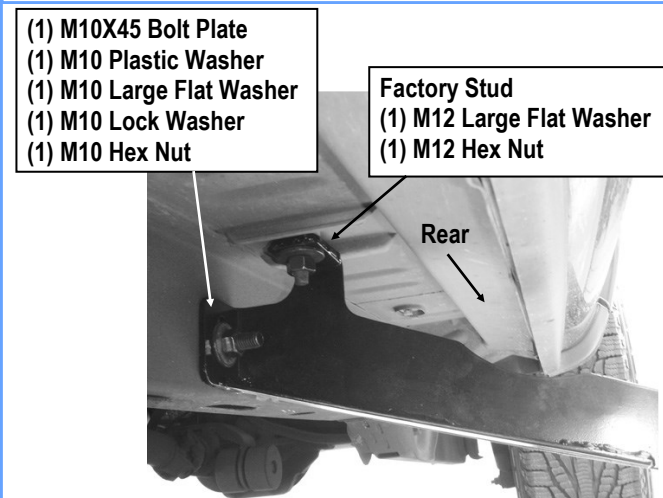
(Fig 7) Driver Rear Mounting Bracket Installation
