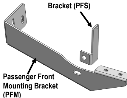
Passenger Front Support Bracket (PFS)
