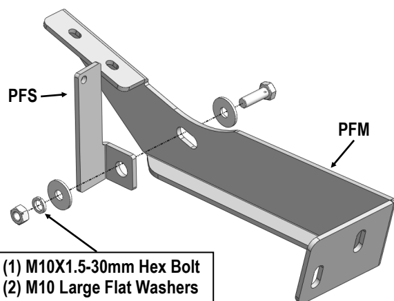
(Fig 4) Passenger Front Mounting Bracket Assembly
