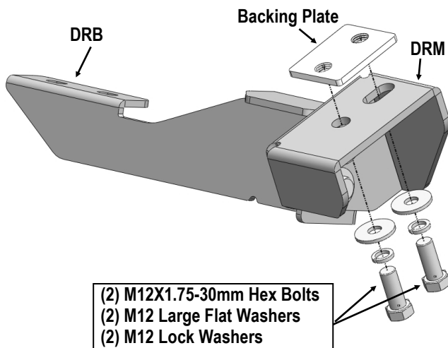
(Fig 6) Driver Rear Mounting Bracket Installation
