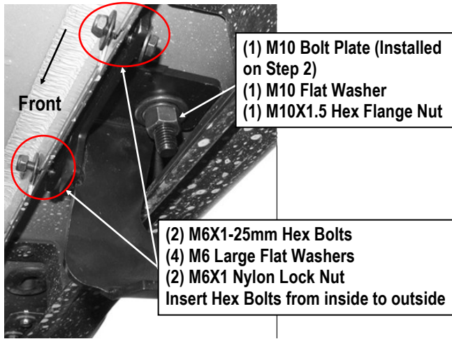
(Fig 5) Passenger Front Mounting Bracket Installation
