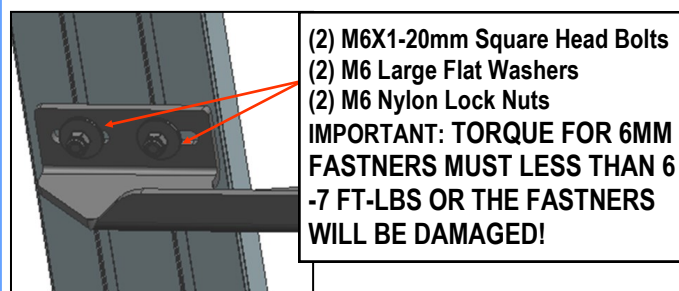
(Fig 8) Running Board Installed Onto Mounting Bracket
