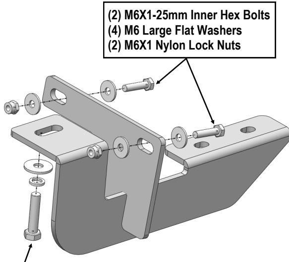
(Fig 3) Passenger Front Mounting Bracket (PFM) Installed
