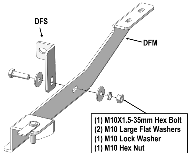
(Fig 3) Driver Front Support Bracket Assembly
