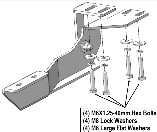
(Fig 4) Driver Rear Bracket Installation
