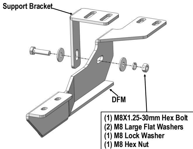
(Fig 3) Driver Rear Brackets Assembly
