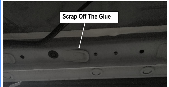
(Fig 3) Driver Side Center Mounting Location Pictured
