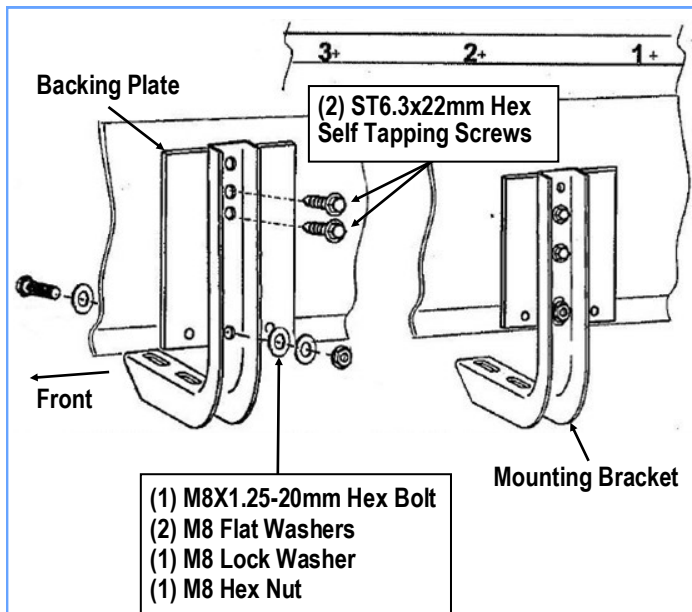
(Fig 2) Passenger Front Mounting Bracket Installation (2nd & 3rd Mounting Bracket Are Same)
