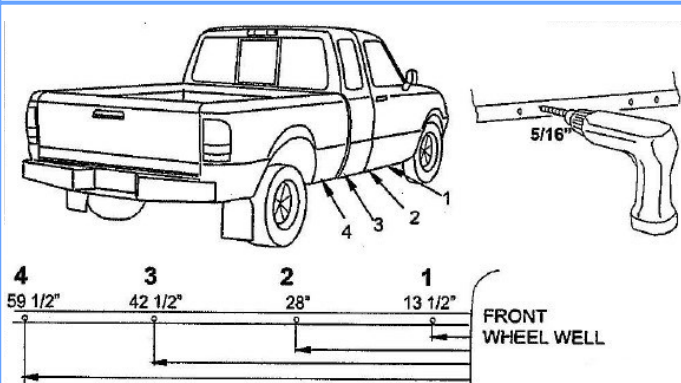
(Fig 1) Passenger Side Mounting Locations
