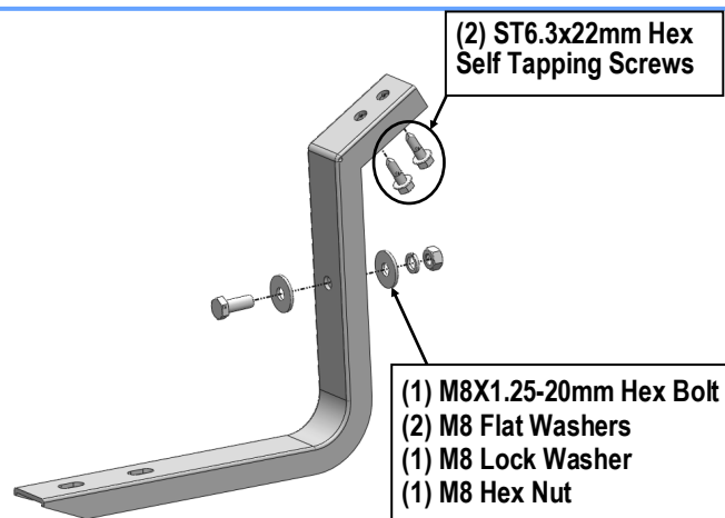
(Fig 3) Passenger Rear Mounting Bracket Installation
