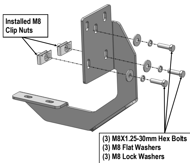
(Fig 3) Driver Rear Mounting Bracket Installation
