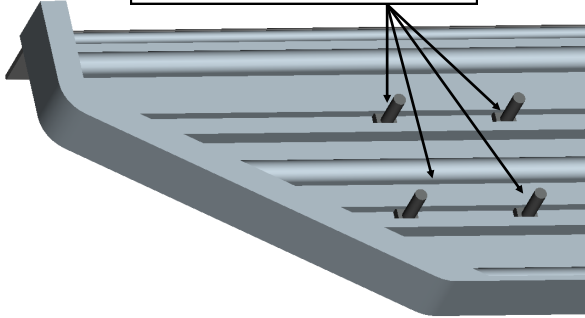
(Fig 7) Slip (3) M6X1-20mm Square Head Bolts Into Each Bottom Channel
