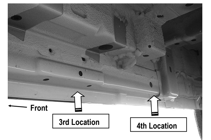
(Fig 13) Passenger Side 3rd Mounting Bracket Location
