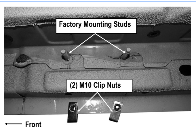
(Fig 12) Passenger Side 2nd Mounting Bracket Location
