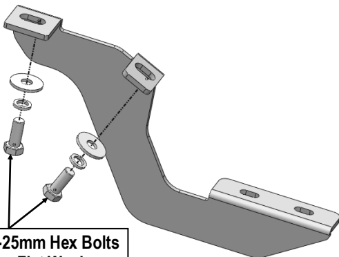
(Fig 2) Passenger Front Mounting Bracket Installation
