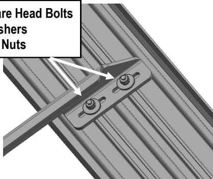
(Fig 5) Running Board Installed Onto Mounting Bracket
